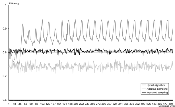
Fig. 2. Comparison of the various download policies over time
