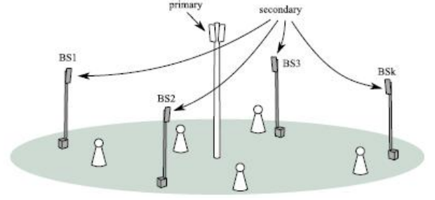
Figure 3. Sensing Scenario [8]
