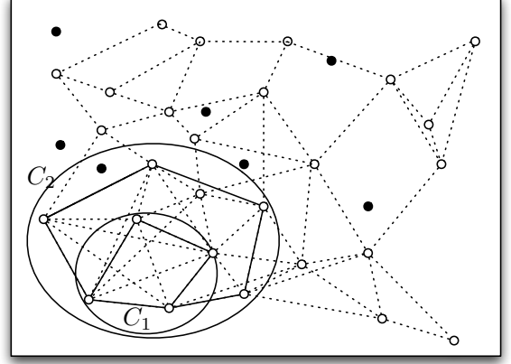
Figure 4. C_1 is the maximum region formed by r = r_{min} in algorithm 1. C_2 is the maximum region in the second stage of algorithm 1 where r = r_{min} + \delta
