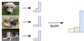
Similar labels sum to give focussed distribution
