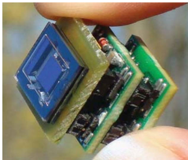
FOREVER NODE: Imec created this energy-harvesting wireless sensor. PHOTO: IMEC
